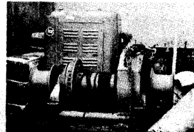
Mooring Winch
