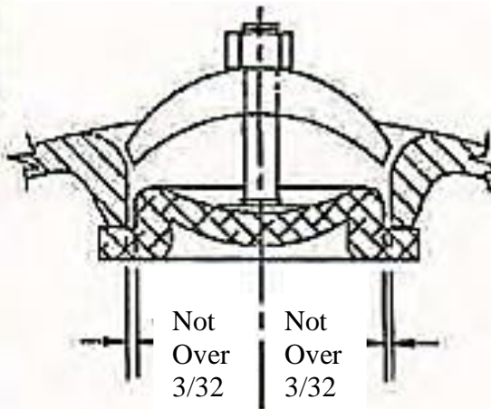
MANHOLE CLEARANCE
