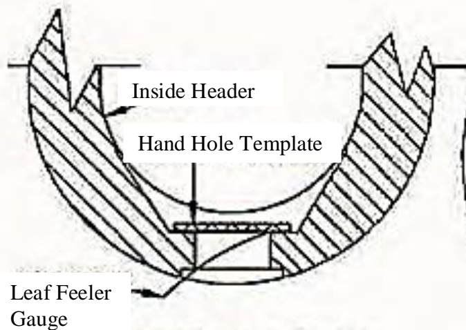
SEAT TAPER
