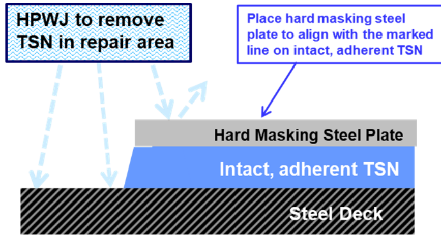
Figure B-1: Cross section view of masking alignment for TSN removal using HP WJ
