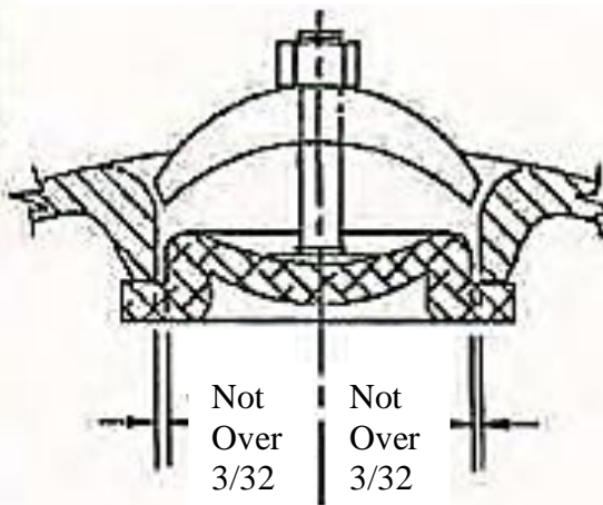
MANHOLE CLEARANCE
