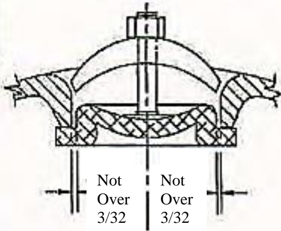
MANHOLE CLEARANCE
