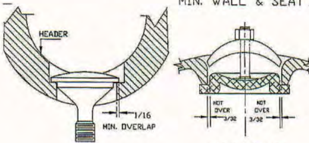
MANHOLE CLEARANCE
