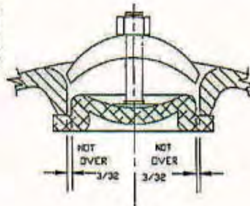
MANHOLE CLEARANCE
