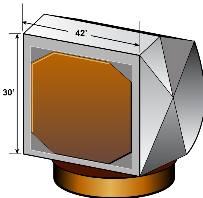
Figure 5. S-Band Antenna
