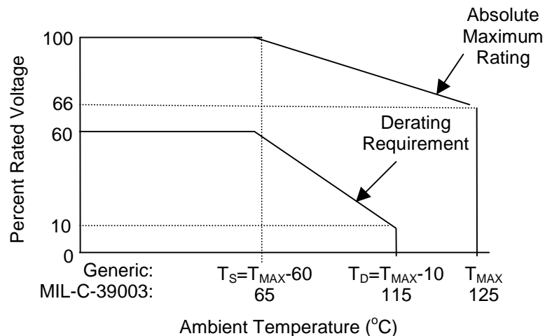
Figure 11. Derating Requirement for Fixed Value, Solid Tantalum Electrolytic Capacitor
