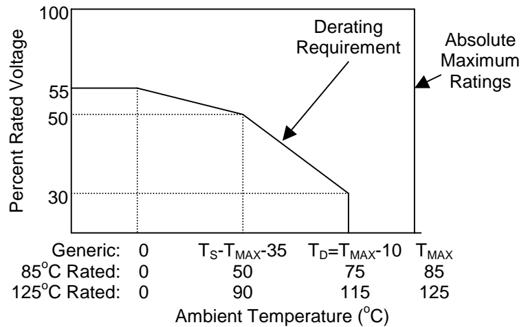
Figure 3. Derating Requirement for Fixed, Metallized Paper, Paper-Plastic, and Plastic Capacitor
