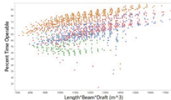
Figure 11 – Design Space percentage time operable for Transit and Patrol Mission in the Gulf of Alaska as a function of prismatic volume
